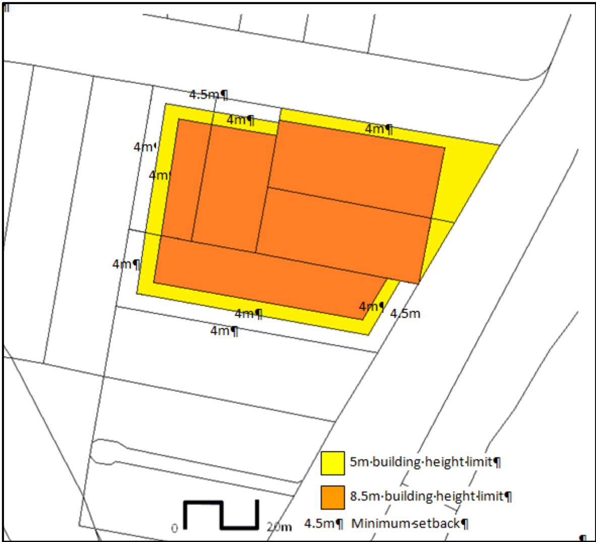
Figure DEV-P1.6.1 - Building envelope as required by subclause DEV-P1.6.1 A1
